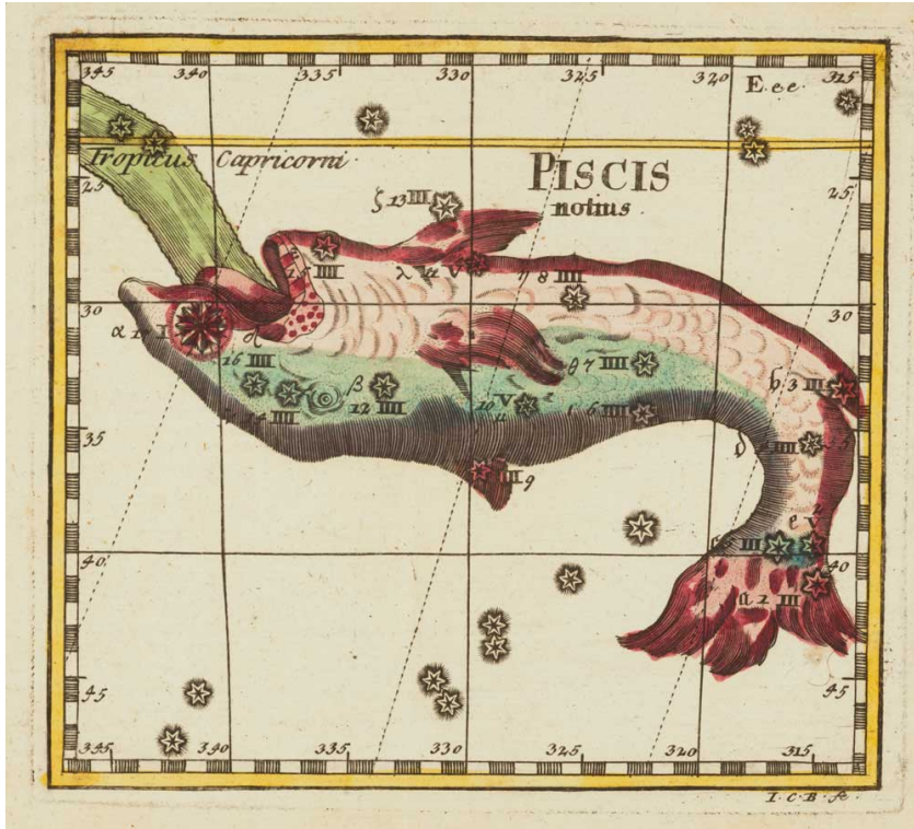
18th century illustration of the constellation Piscis Austrinus
