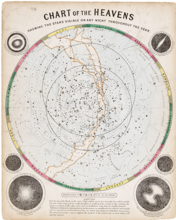
A transparency astronomical chart of the heavens
