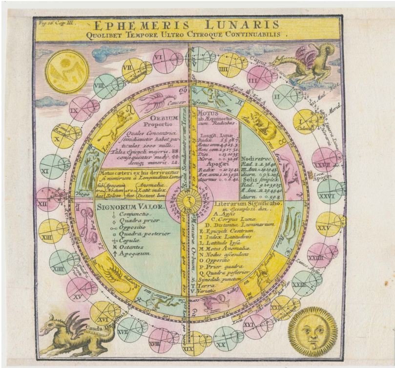
18th century illustration of the phases of the Moon
